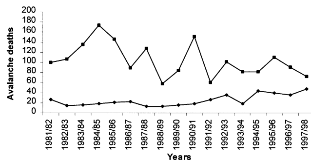
Fig. 1. Annual figures of avalanche deaths in Austria, France, Germany, Italy and Switzerland (■), as well as in Canada and the USA (◆) 1981–1998 [1] ( n total = 2197). No trend is observed in the Alpine countries ( r = -0.29 , P = 0.24 ; Spearman’s correlation coefficient). By contrast, the curve for North America shows an increase in avalanche deaths ( r = 0.68 , P = 0.002 ; Spearman’s correlation coefficient).
